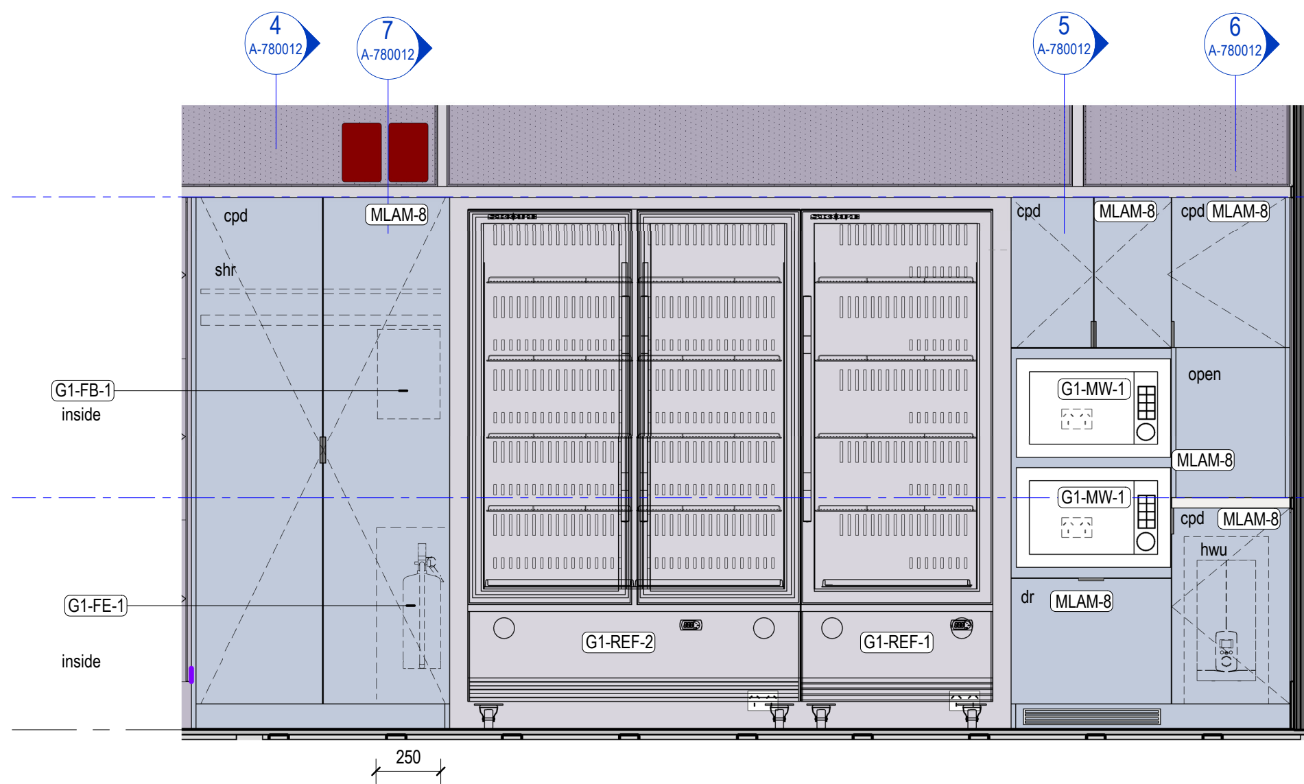
2 JO-ST-2 Elevation 1 : 20
